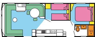
29 X 10 2-bed shower and toilet
